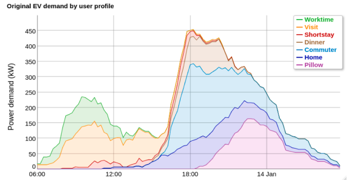
Fig. 11. Original EV power demand by user profile.
